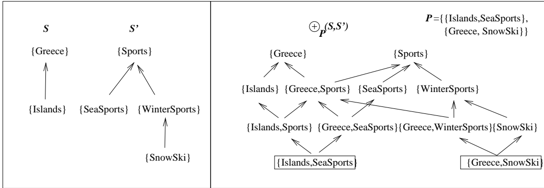
Figure 4: An example of a plus-product , \oplus_P , operation
